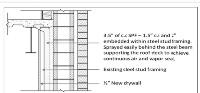
Figure 8: Roof-to-wall junction behind the steel beam sealed effectively with spray foam.
