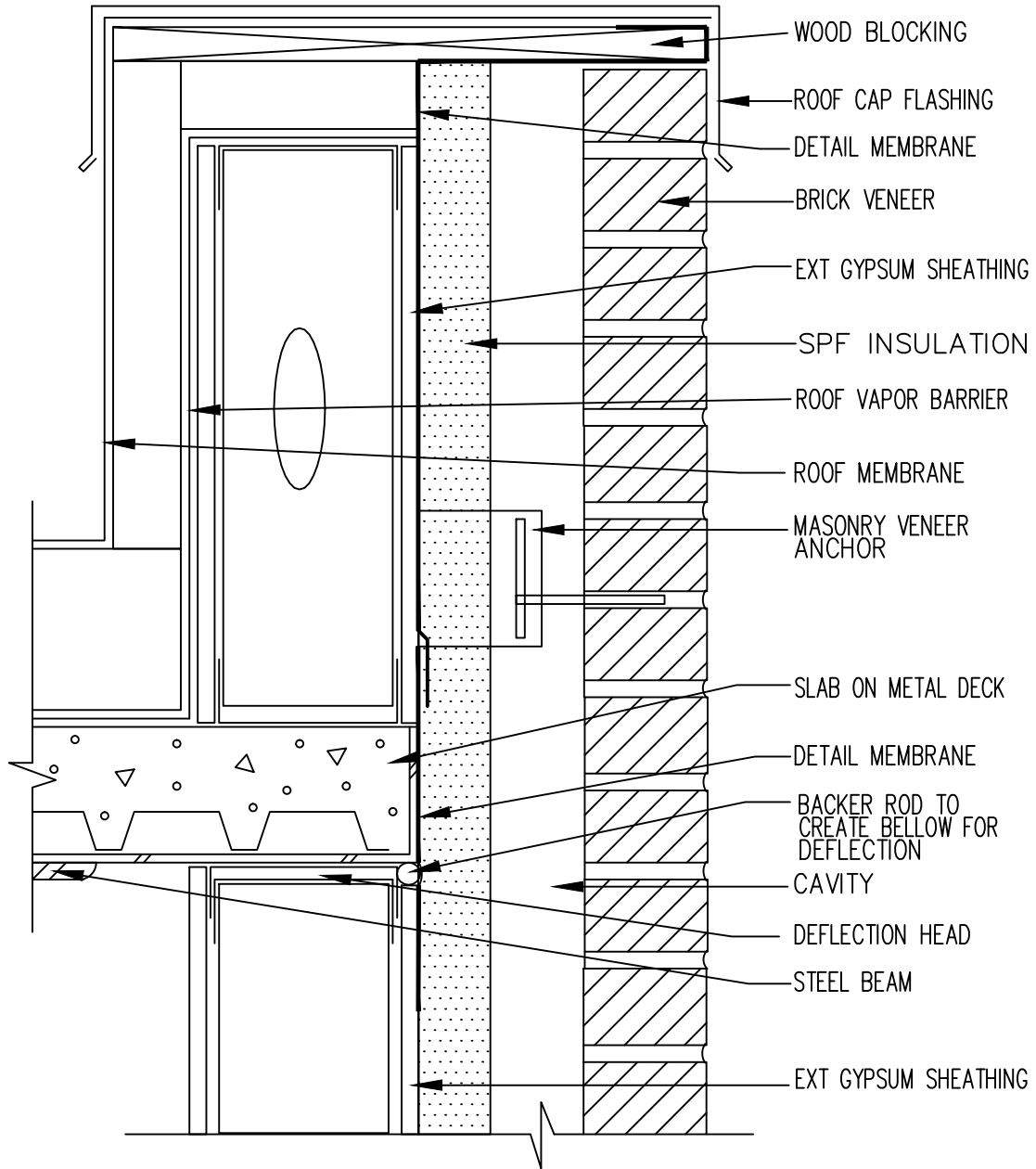
Roof Detail 2 Parapet
