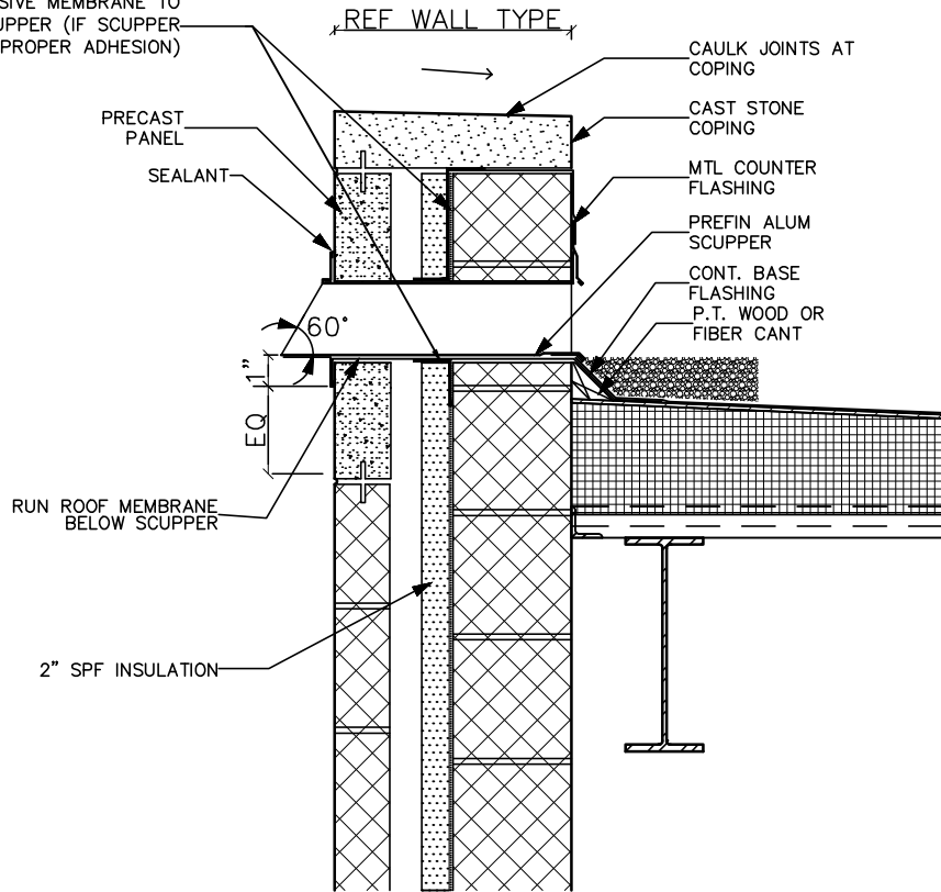
2 TYP PARAPET / OVERFLOW SCUPPER A10.02 1"=1' - 0"
