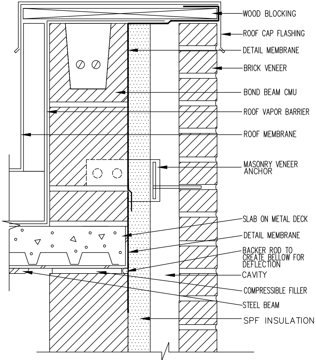
Roof Detail Parapet 1 CMU
