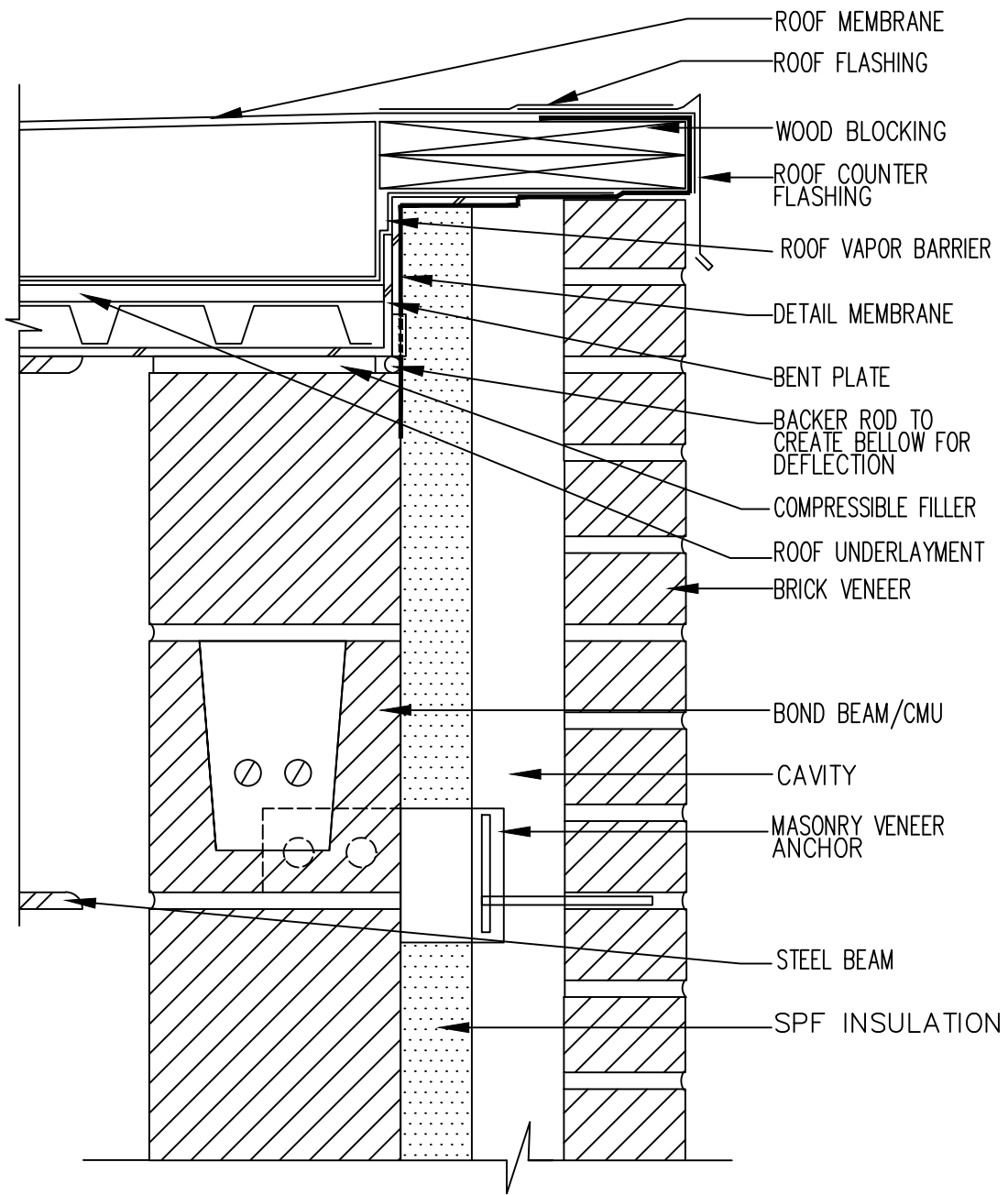
Roof Detail 2 CMU
