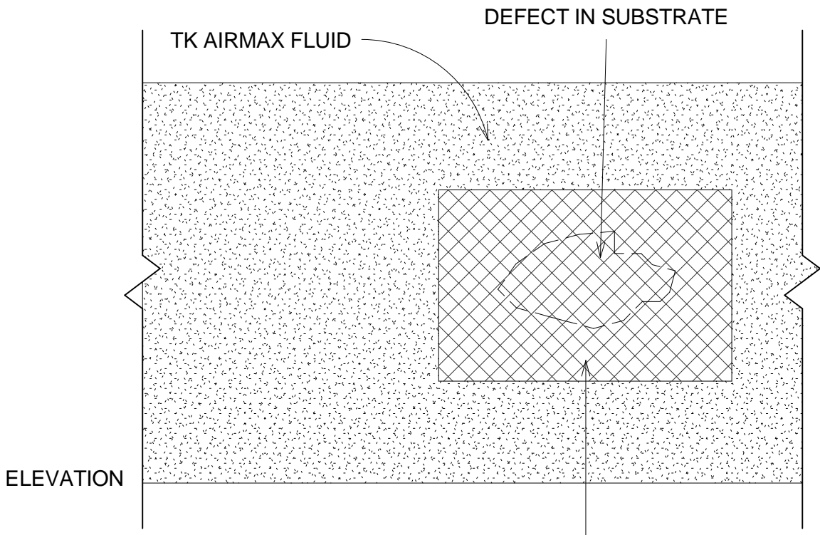
DEFECT COVERED WITH AIRMAX 2200 ALL WEATHER FLASHING
